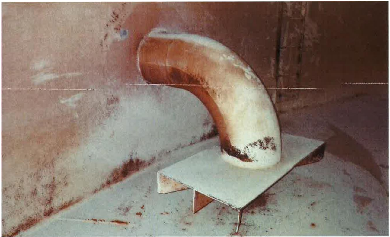
67. Outlet pipe and anti-vortex assembly.
