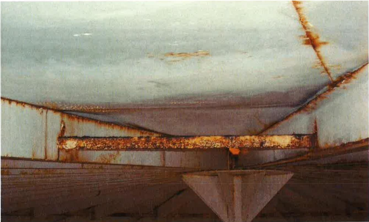
54. Corrosion and metal loss on purlin.
