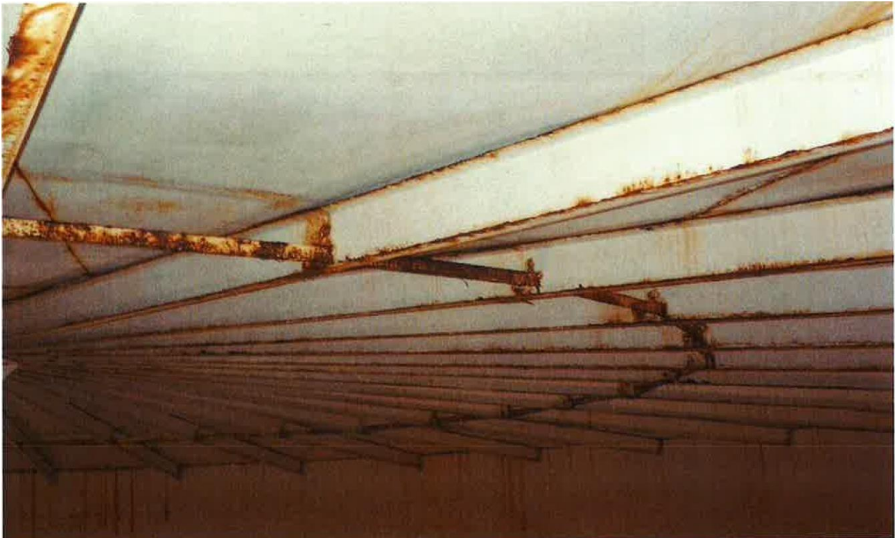
56. Roof support structure. Note corrosion and metal loss.
